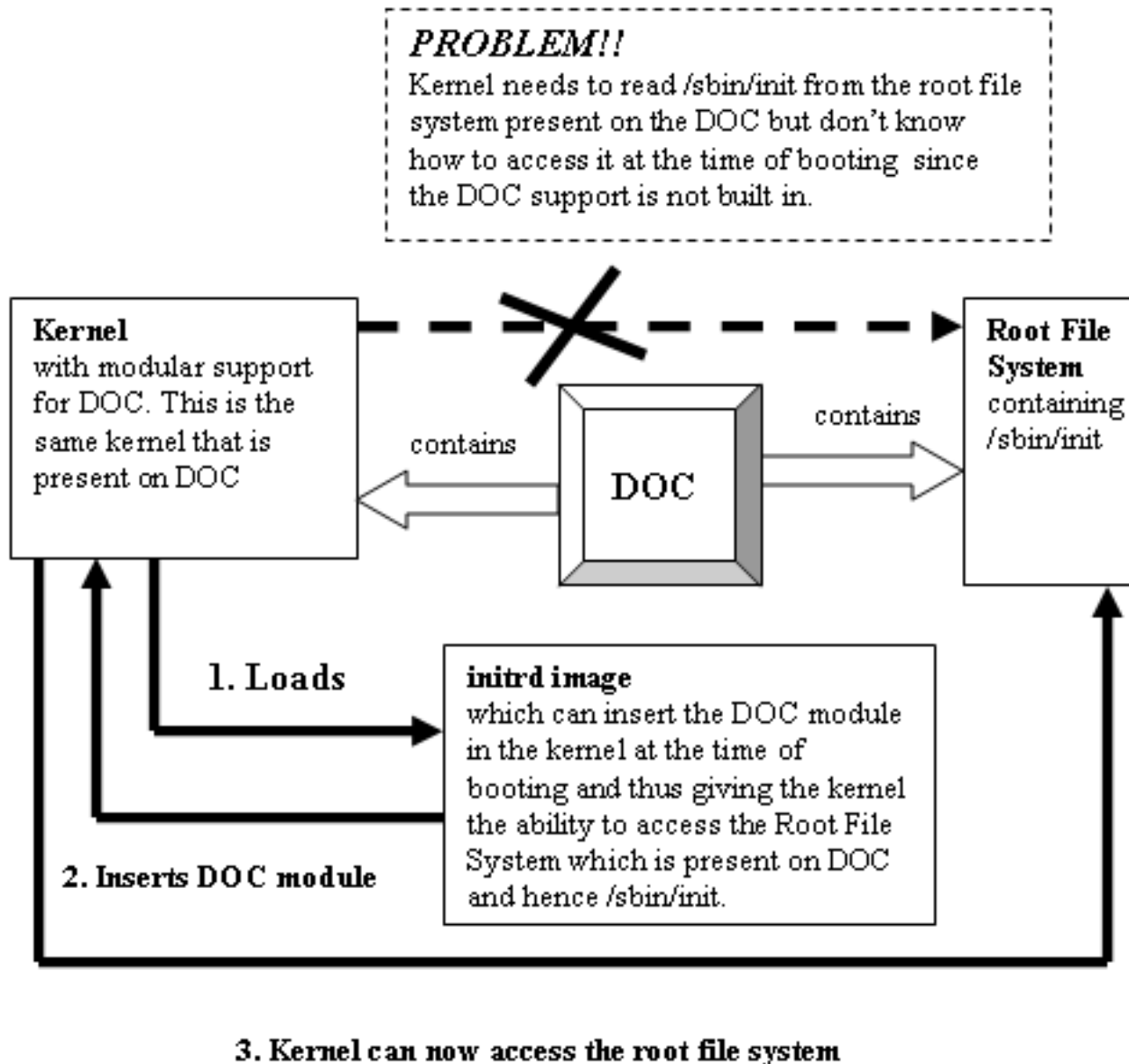
Figure 1. Why we need an initrd image
